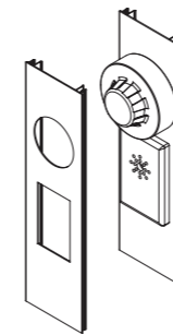
Smoke detector and fire alarm sander (standard duct cover cut-outs)
